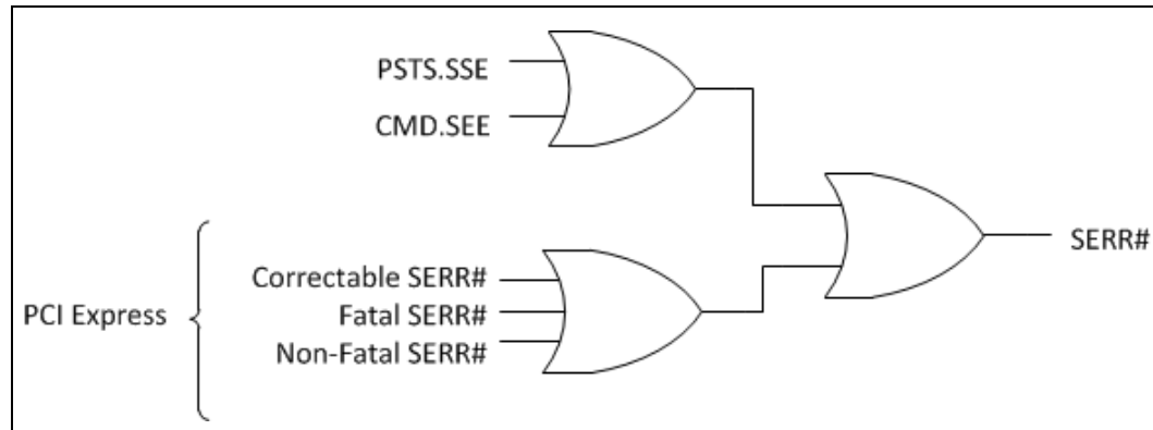
Figure 5-2. Generation of SERR# to Platform
